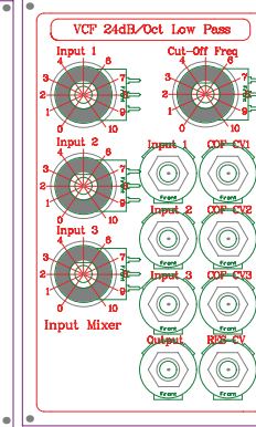
VCF
