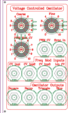
VC01
