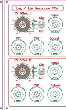
VCA x 2
